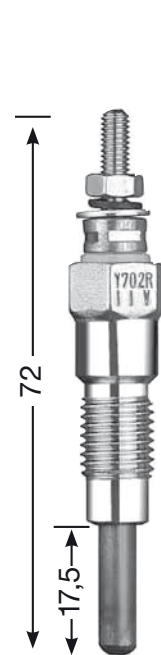
Y-702 R M 10 x 1.25 12 Hex 11 V
