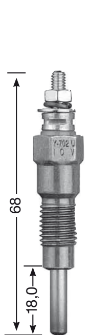
Y-702 U M 10 x 1.25 12 Hex 10 V
